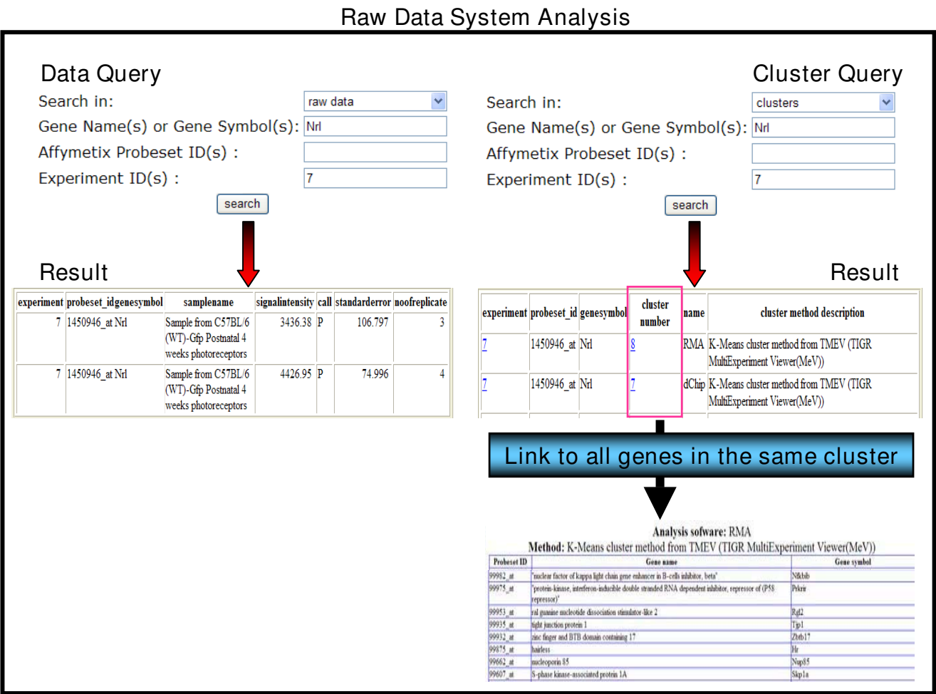
Figure 3 Data and Cluster Query options. Data and cluster query results for the NRL gene in experiment 7 [17]: "Targeting GFP to new born by NRL promoter and temporal expression profiling of flow-sorted photoreceptors". The user can subsequently obtain all genes present in the given cluster.
